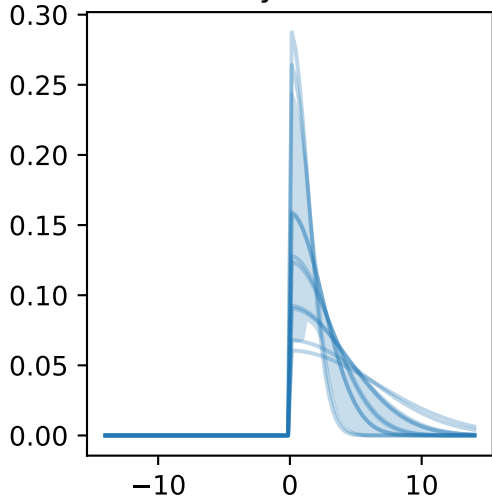
event=PyData-Berlin
